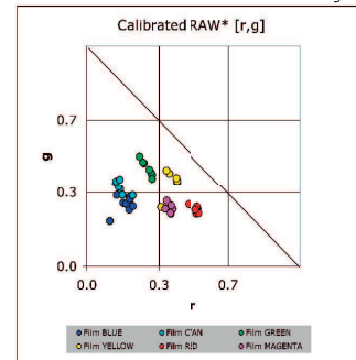
Figure 9. RAW* Chromaticities of the ColorChecker® squares in variable exposures. Each color point is the plot for different exposures of color papers using RAW* color separation values with linear calibration.
