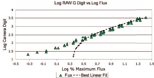
Figure 12 replots the data in Figure 11 using log log axes. The lower half of the logarithmic range departs from the linear fit. The upper half falls slightly below the linear fit.
